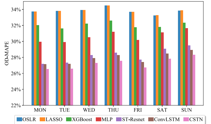
Fig. 6. The MAPE of different methods for taxi origin-destination demand prediction on different days of the week. Our method consistently outperforms the other methods in all days of the week.
