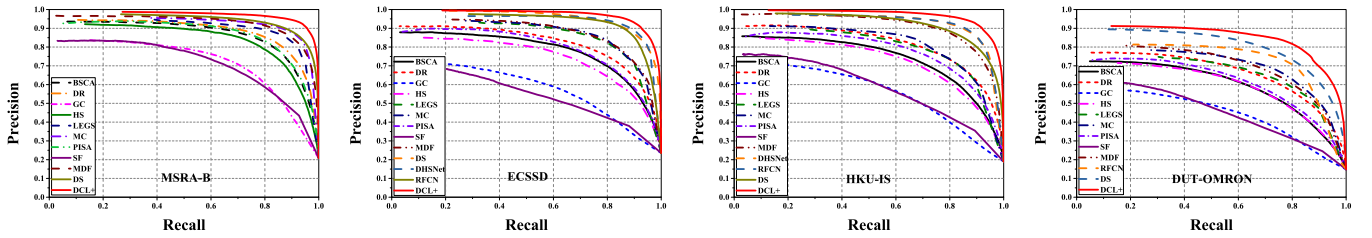
Fig. 5. PR curves of our method and 12 other state-of-the-art algorithms on 4 benchmark data sets. Our DCL + (DCL with CRF) consistently performs better than other methods across all the benchmarks.
