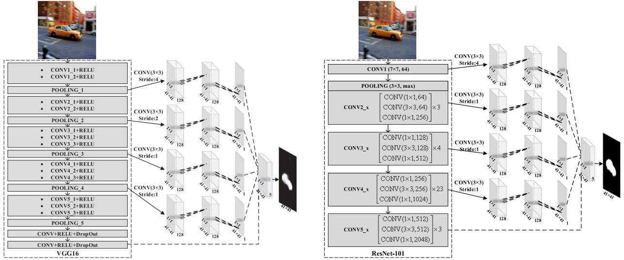
Fig. 2. Architecture of VGG-16-based MS-FCN (left) and ResNet-101-based MS-FCN (right). We connect three extra convolutional layers to each of the first four max-pooling layers of VGG-16 and convert it to a multiscale version. For ResNet-101, we divide the 101 layers into five groups and connect an extra subnetwork with three convolutional layers to each of the final layers in the first four groups to form the multiscale version.
