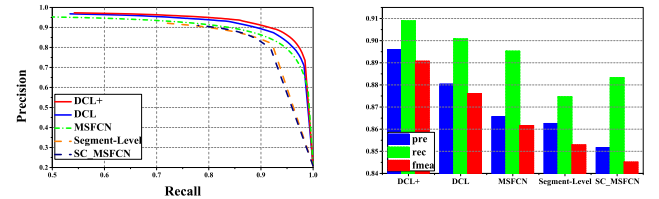
Fig. 7. Componentwise validation of the proposed model and the effectiveness of CRF-based refinement.
