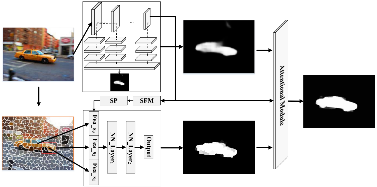
Fig. 1. Overall architecture of our proposed contrast-oriented deep neural network. It consists of a fully convolutional stream (top), a segmentwise SP stream (bottom), and an attentional module to fuse the intermediate saliency maps from the two streams. “SFM” refers to the segment feature masking layer, while “SP” refers to the SP operation.
