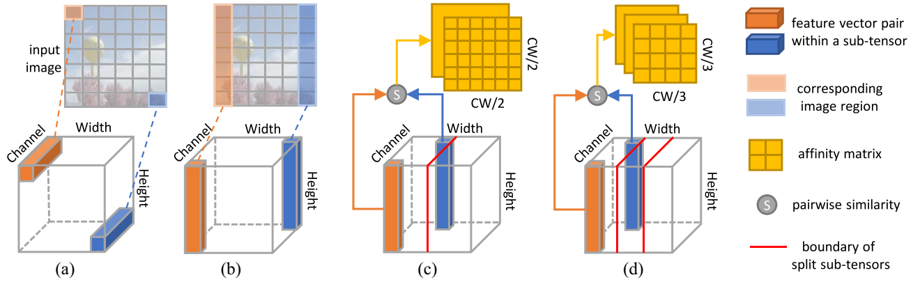
Fig. 4. (a) Vanilla (spatial) nonlocal module. (b) Vanilla DNL module (vertical-split). (c) Divide-and-conquer DNL module (vertical-split, split number, s = 2 ). (d) Split number, s = 3 . Dense pairwise similarity is computed between each pair of feature vectors (the orange bar and the blue bar) within the same region/subregion. In (c), the C \times W plane is split into two subregions.
