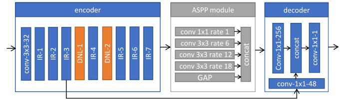
Fig. 5. Depthwise nonlocal deep neural network. As shown in the above, IR denotes the IR module while DNL denotes the DNL module. “Rate” refers to the dilation rate of a convolution. GAP denotes global average pooling.
