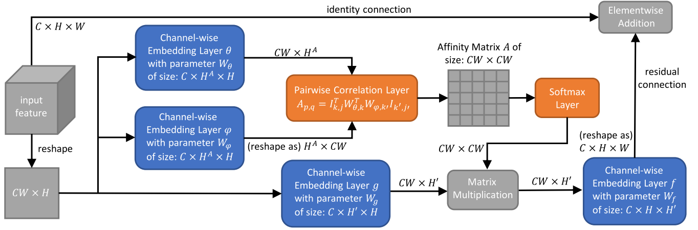
Fig. 3. Vanilla DNL module (vertical-split). The proposed module contains four channel-wise embedding layers, a pairwise correlation layer, and a softmax layer. The softmax layer normalizes each row of the affinity matrix A . The matrix multiplication serves as taking the weighted summation of the output of layer g , with the softmax output as attention weights.
