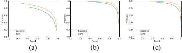
Fig. 8. Ablation study on precision-recall curves. In the above graphs, the blue curve denotes the baseline model without deploying any proposed modules, while the orange one denotes our proposed DNL network. Our proposed method obtains higher precision than the baseline, for the same recall value. (a) DUT-O. (b) ECSSD. (c) HKU-IS.
