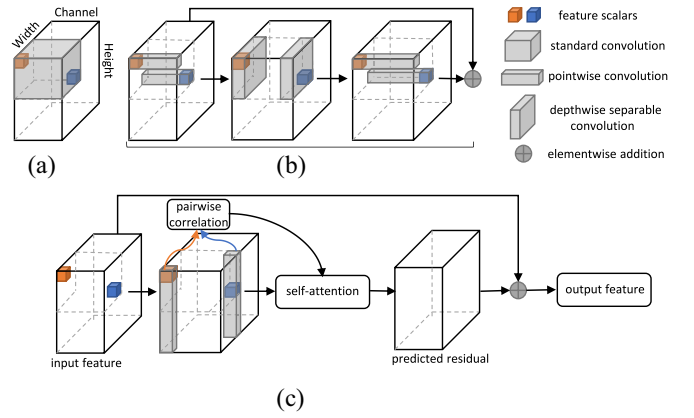
Fig. 2. (a) Standard Convolution. (b) IR. Before the elementwise addition in IR, the shapes of the two feature maps are aligned with each other. Note that the correlation of two spatially close scalars (in orange and blue colors, respectively) is not directly captured in an IR, while a standard convolution can predict outputs based on them together. (c) Our proposed DNL module. The proposed module can capture the correlation between two feature vectors, which are located at different channels and spatial positions.
