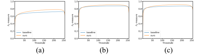
Fig. 9. Ablation study on threshold- F_\beta measure curves. As shown in the above, the F_\beta measures of our proposed method are considerably higher than those of the baseline, for most thresholds within the range of [50, 200]. (a) DUT-O. (b) ECSSD. (c) HKU-IS.
