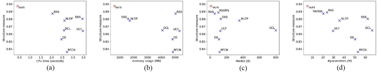
Fig. 7. Comparisons on efficiency and quality. To measure the efficiency and quality of salient object detection models at the same time, the above scatter diagrams take an efficiency metric as horizontal axis and a quality metric as vertical axis. Our proposed method is always located at the upper left of these diagrams, which indicate the best tradeoff between efficiency and accuracy. (a) Smeasure-CPU time. (b) Smeasure-Mem. (c) Smeasure-MAdds. (d) Smeasure-Params.
