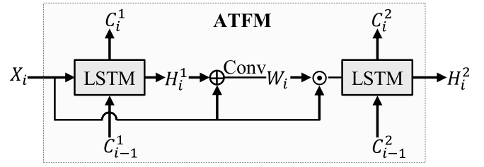
Fig. 2. Overview of the proposed Attentive Traffic Flow Machine (ATFM). X_i is the normal traffic flow feature of the i^{th} iteration. “ \oplus ” denotes a feature concatenation operation and “ \odot ” refers to an element-wise multiplication operation. The first ConvLSTM unit takes X_i as input and incorporates the historical information to dynamically generate a spatial attention map W_i . The second ConvLSTM unit learns a more effective spatial-temporal feature representation from the attentionally weighted traffic flow features.
